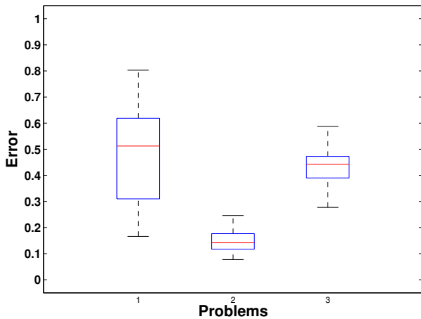
Fig. 4. Boxplot analysis of NS-GP-R performance on each benchmark problem, showing the best test-set error achieved in each run.
